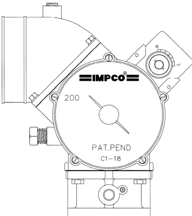
Original design, featuring a hex idle adjustment screw.
